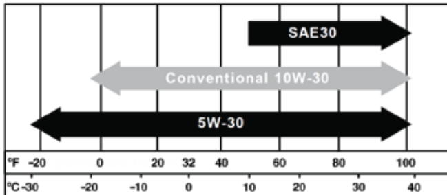
Figure 1 - Recommended Oil
